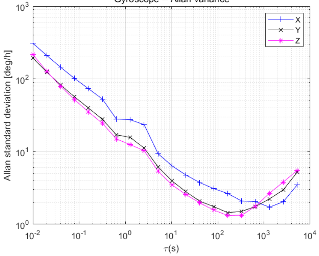
Gyroscope -- Allan variance
